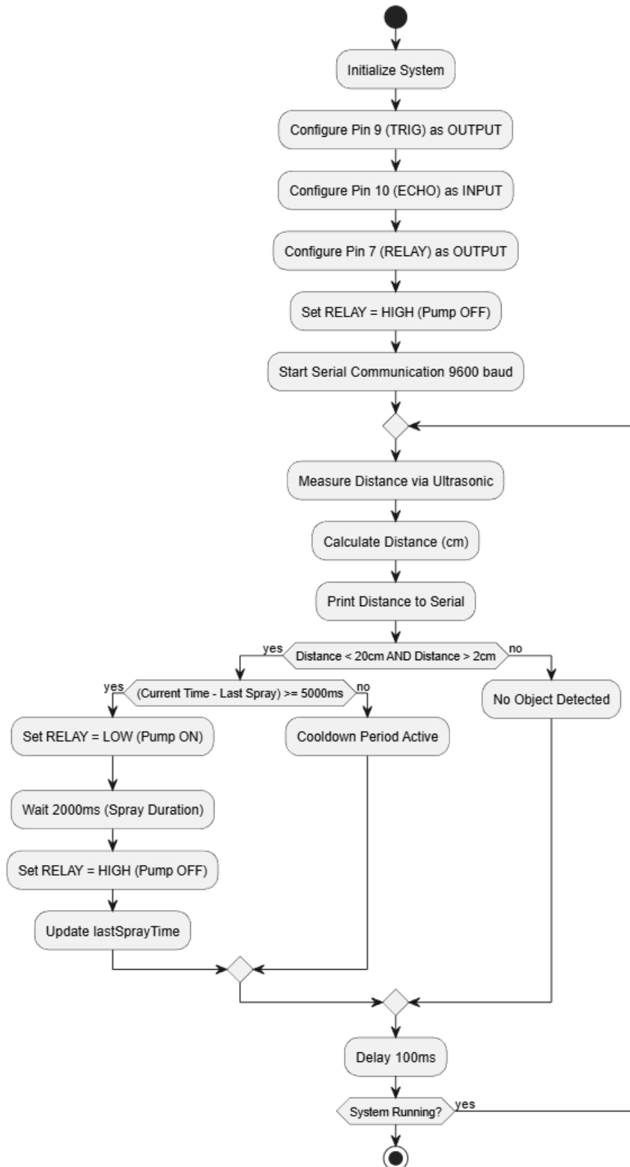
Figure 11: Software Control Flow Diagram
