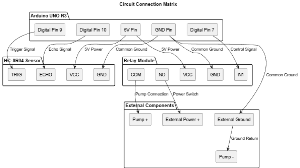
Figure 10: Circuit Connection Matrix
