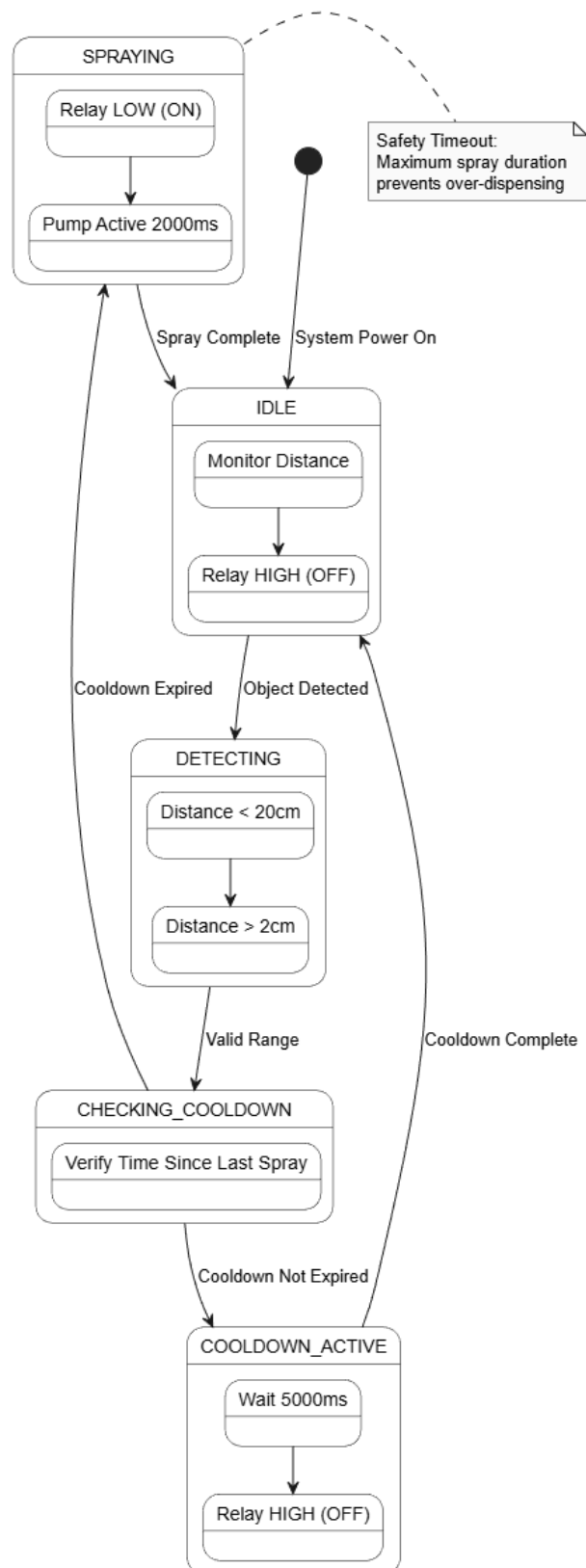
Figure 14: State Machine Diagram
