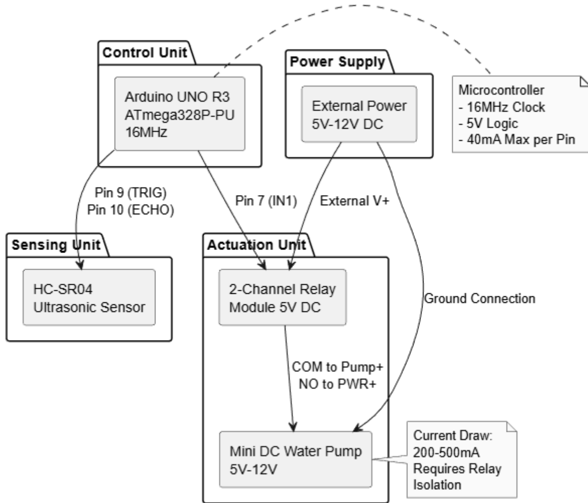
Figure 9: System Architecture Diagram
