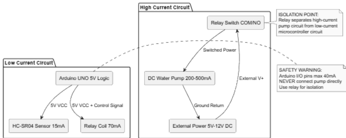
Figure 13: Power Distribution and Safety Diagram
