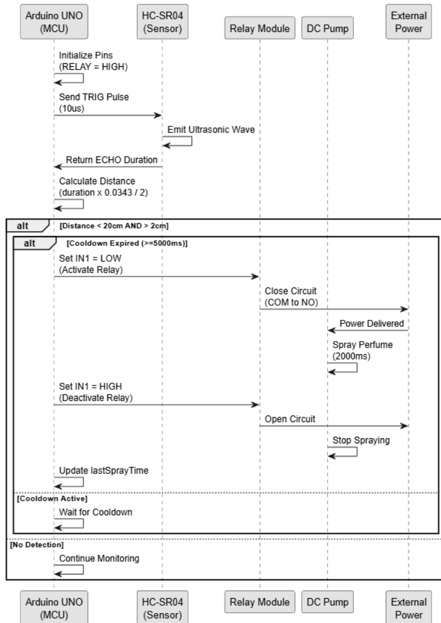
Figure 12: Component Interaction Sequence Diagram
